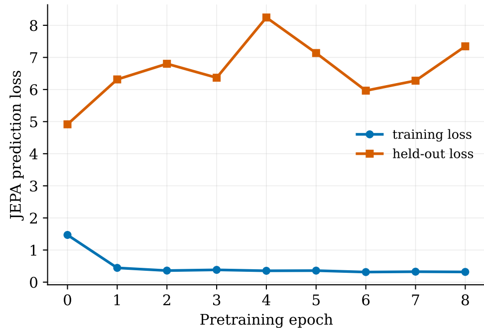
Self-supervised pretraining
