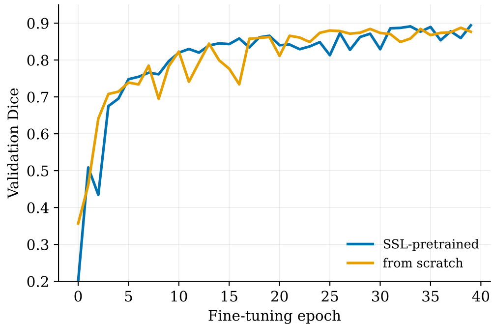
Fine-tuning (100\% labels)
