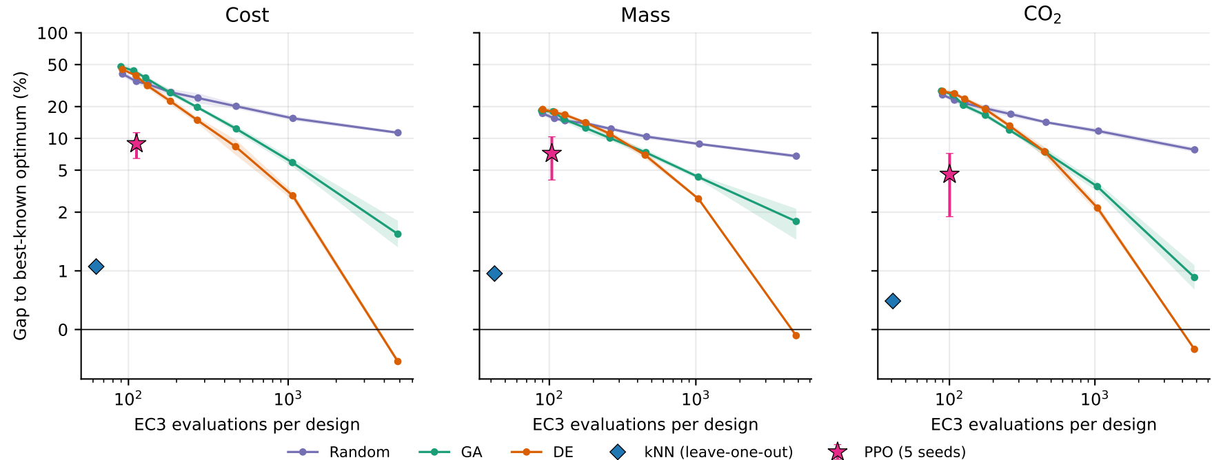
Main grid, scale+thin: per-context search ( B = 20 \dots 4800 , evaluations include the operators) vs amortized methods
