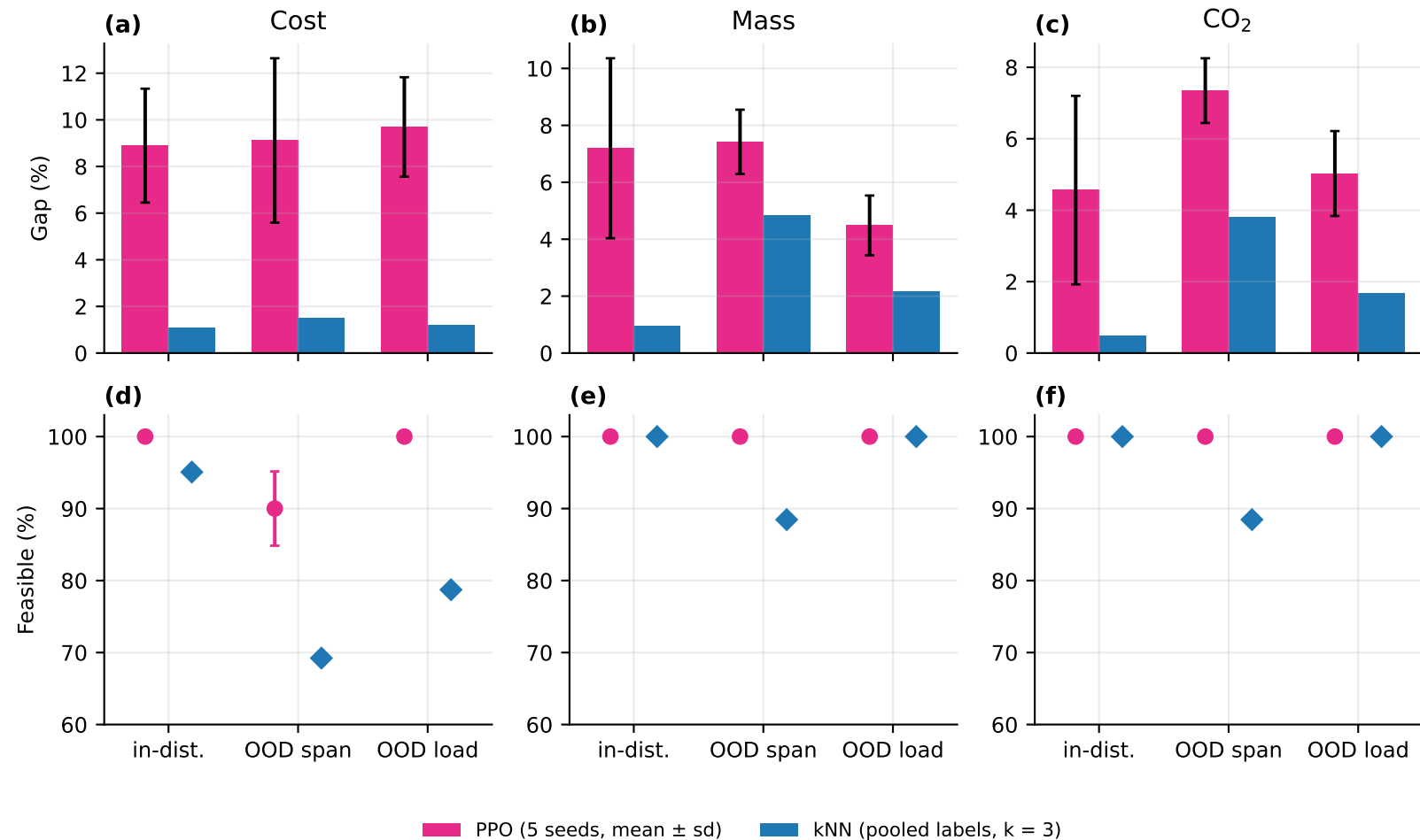
In-distribution vs out-of-distribution (scale+thin; OOD = contexts with a feasible reference only)
