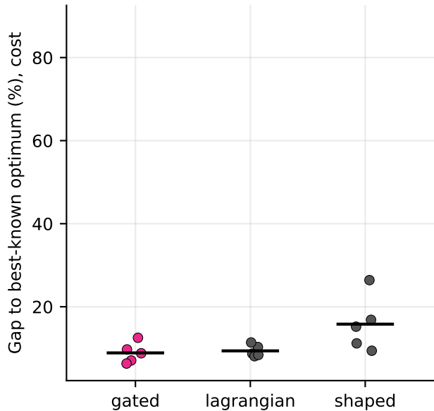
2a: PPO reward mode
