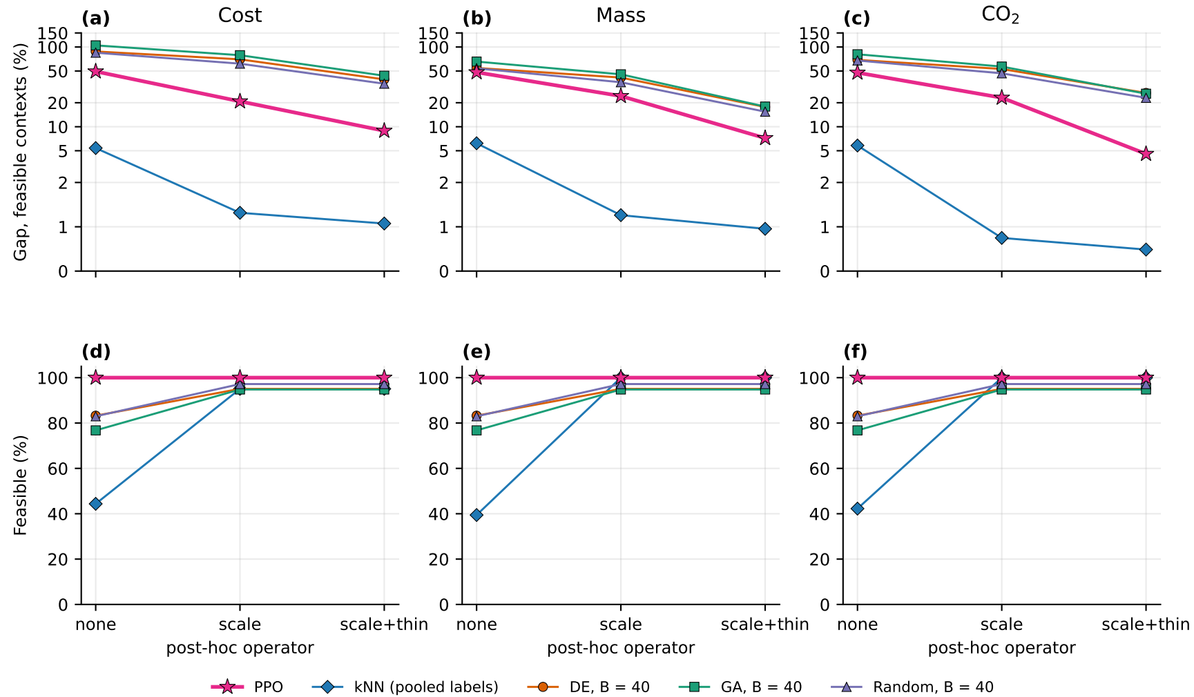
Effect of the post-hoc operator on every method (main grid; searches at B = 40)
