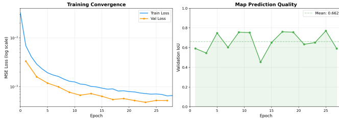
Fig. 2. Training convergence (left) and validation IoU (right) over 29 epochs. Loss decreases smoothly from 0.033 to about 0.0007 over training, with only minor sub-0.001 fluctuations in the late epochs.
