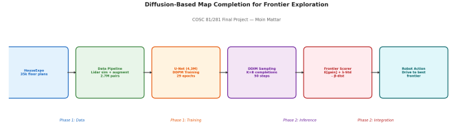
Fig. 1. System pipeline. HouseExpo floor plans drive synthetic data generation via lidar simulation. The trained U-Net performs conditional denoising to complete partial maps; multiple completions score frontiers for autonomous exploration in ROS 2 / Stage.
