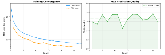
Fig. 2. Training convergence (left) and validation IoU (right) over 29 epochs. Loss decreases monotonically from 0.033 to 0.0007 with no instabilities, the diffusion-training stability story playing out at our scale.
