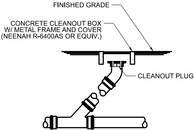
CLEANOUT IN PAVED AREAS NOTE: G.C. IS TO INSTALL CLEANOUT AT ANY PIPING ANGLE CHANGES AND EVERY 50' IN PIPING RUNS GREATER THAN 100' IN LENGTH
