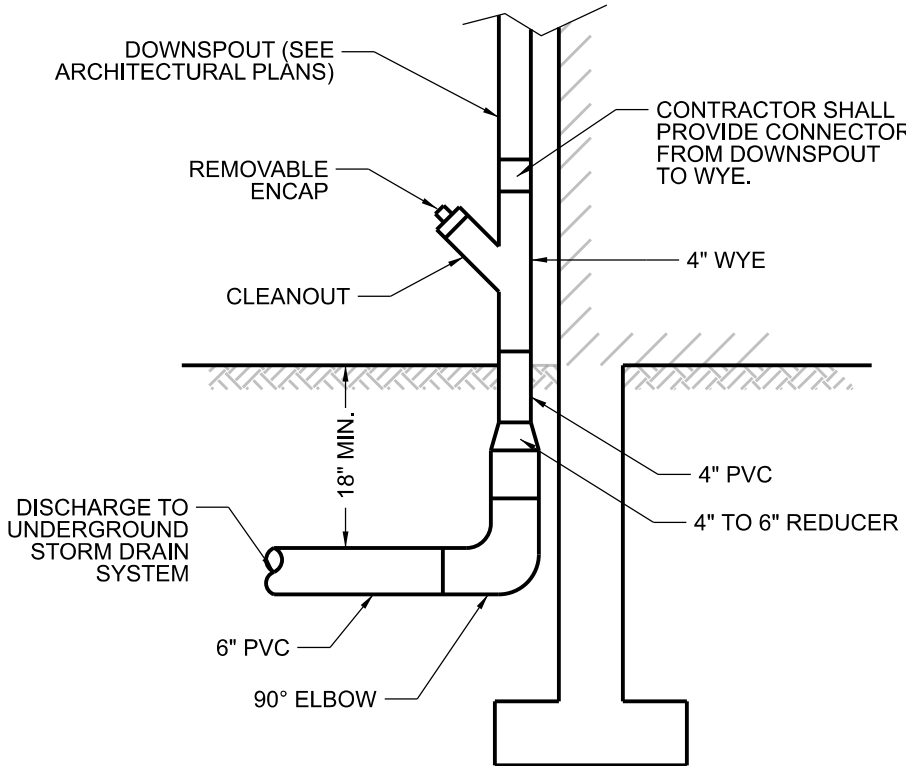
DOWNSPOUT CONNECTION NOT TO SCALE
