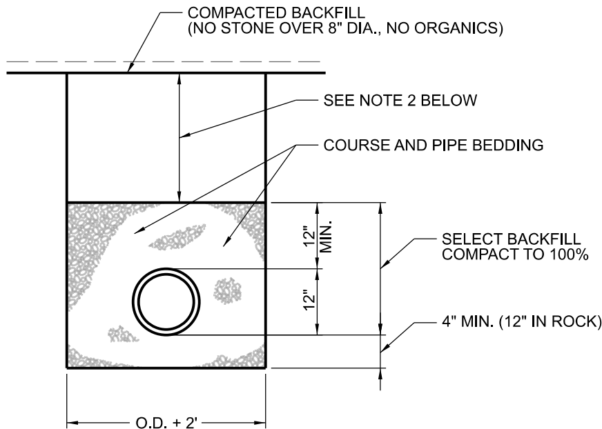
SANITARY SEWER BEDDING TO COMPLY WITH COUNTY STANDARDS SCALE: 1/2"=1'-0"
