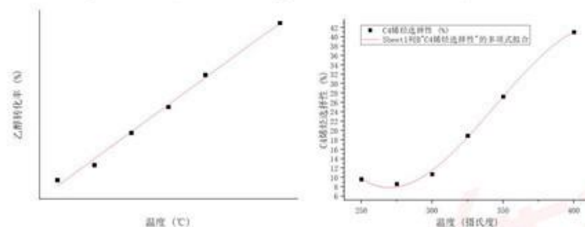
A4: 200mg 0.5wt%Co/SiO 2 - 200mg HAP-乙醇浓度 1.68ml/min
