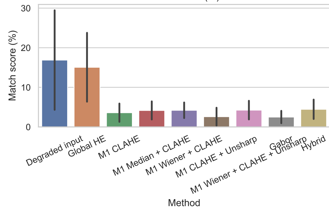
Match score (%)
