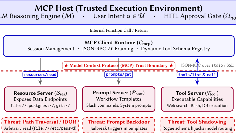
Fig. 3. Model Context Protocol (MCP) architecture and trust boundaries. The Host and Client form the Trusted Computing Base (TCB), communicating via JSON-RPC 2.0 with external, semi-trusted MCP servers across the boundary. Red dashed boxes highlight primary attack surfaces: URI path traversal in resource reads, prompt backdoor injection in workflow templates, and tool shadowing during dynamic capability registration.
