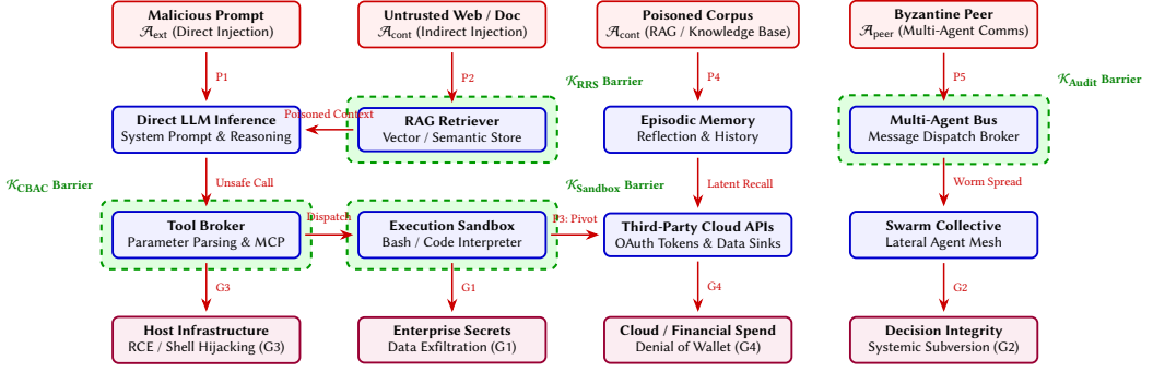
Fig. 2. Causal threat graph of exploit propagation paths (P1–P5) to target assets (G1–G4). Red nodes indicate adversary footholds, blue nodes show internal execution components, and purple nodes denote target assets. Green dashed contours mark interdiction barriers that sever the kill chain.
