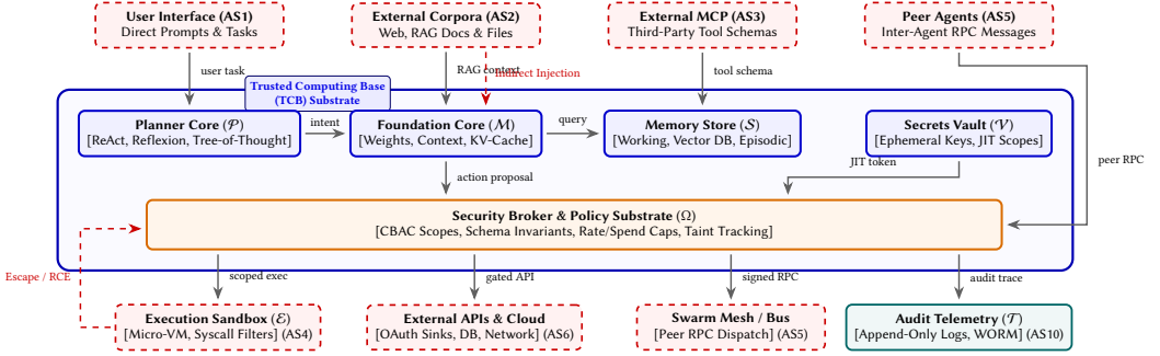
Fig. 1. Agentic AI reference architecture and Trusted Computing Base (TCB) delineation. Blue boxes denote verified TCB modules ( \mathcal{P}, \mathcal{M}, \mathcal{S}, \Omega ), while dashed red containers highlight untrusted ingress and execution surfaces. Gray arrows trace capability flows mediated by security broker \Omega ; dashed red vectors indicate prompt injection and sandbox escape paths.
