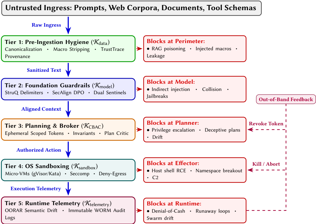
Fig. 5. Defense-in-depth framework across five operational tiers ( \mathcal{K}_{\text{data}} to \mathcal{K}_{\text{telemetry}} ). Solid arrows show request traversal through mediation layers, red badges denote intercepted threats, and dashed purple lines trace out-of-band feedback for dynamic credential revocation.
