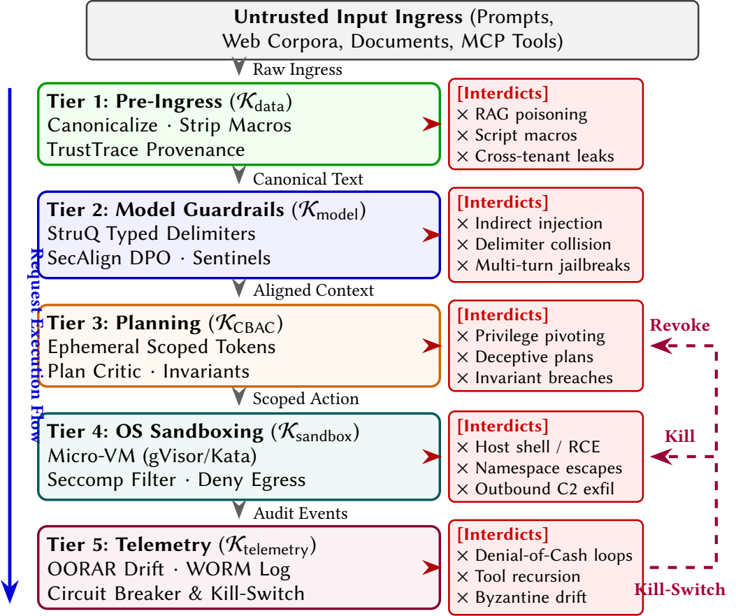
Fig. 5. Defense-in-depth framework across five operational tiers ( \mathcal{K}_{data} to \mathcal{K}_{telemetry} ). Solid arrows show request traversal through mediation layers, red badges denote intercepted threats, and dashed purple lines trace out-of-band feedback for dynamic credential revocation.
