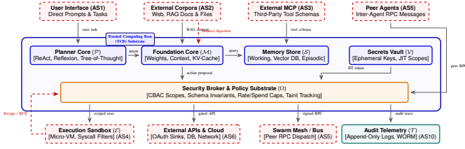
Fig. 1. Agentic AI reference architecture and Trusted Computing Base (TCB) delineation. Blue boxes denote verified TCB modules ( \mathcal{P}, \mathcal{M}, \mathcal{S}, \mathcal{V} ), while dashed red containers highlight untrusted ingress and execution surfaces. Gray arrows trace capability flows mediated by security broker \Omega ; dashed red vectors indicate prompt injection and sandbox escape paths.
