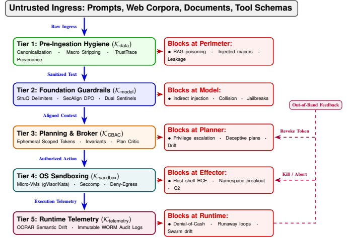
Fig. 5. Defense-in-depth framework across five operational tiers ( \mathcal{K}_{\text{data}} to \mathcal{K}_{\text{telemetry}} ). Solid arrows show request traversal through mediation layers, red badges denote intercepted threats, and dashed purple lines trace out-of-band feedback for dynamic credential revocation.
