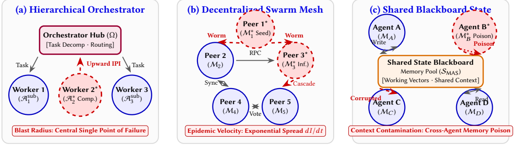
Fig. 4. Multi-Agent System (MAS) coordination topologies and vulnerability propagation dynamics across three canonical architectures: (a) Hierarchical Orchestrator, (b) Decentralized Swarm Mesh, and (c) Shared Blackboard. Rounded background cards delineate topological trust boundaries; red dashed circles with asterisks (*) mark compromised/adversarial agents; solid arrows indicate legitimate task dispatches and state updates; dashed and dotted red vectors trace exploit mechanics (Upward Prompt Injection, self-replicating prompt worms, and asynchronous state poisoning). Hierarchical systems concentrate catastrophic risk at the central orchestrator, peer meshes foster exponential prompt-worm propagation ( dI/dt ), and shared blackboards subject all downstream consumers to persistent memory corruption.
