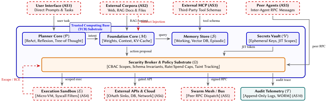
Fig. 1. End-to-end architectural taxonomy and Trusted Computing Base (TCB) delineation for agentic AI systems. Thick blue borders and shaded substrate denote verified TCB components ( \mathcal{P}, \mathcal{M}, \mathcal{S}, \mathcal{V}, \Omega ); red dashed containers designate untrusted ingress surfaces (AS1, AS2, AS3, AS5) and execution targets (AS4, AS6). Solid gray arrows trace authenticated capability and data flows, while dashed red arrows depict adversarial indirect injection and sandbox privilege escalation. Interposing the security broker \Omega enforces capability-based access control (CBAC) and schema invariants prior to all environment side effects.
