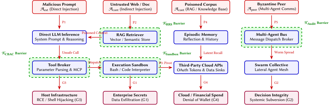
Fig. 2. Causal Threat Graph modeling end-to-end exploit propagation across canonical paths P1, P2, P3, P4, and P5 toward high-value target assets G1–G4. Red boxes denote adversary footholds; blue containers represent internal reasoning and execution substrates; purple boxes represent impact assets. Solid red arrows depict exploit vectors; green dashed contours designate defense interdiction cut barriers positioned on the background layer to sever the kill chain prior to environmental impact.
