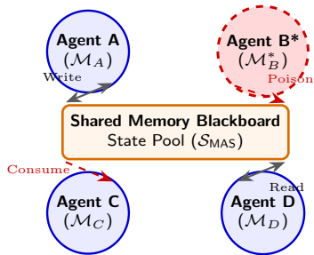
(c) Shared Blackboard
