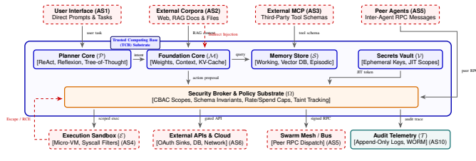
Fig. 1. End-to-end architectural taxonomy and Trusted Computing Base (TCB) delineation for agentic AI systems. Thick blue borders and shaded substrate denote verified TCB components ( \mathcal{P}, \mathcal{M}, \mathcal{S}, \mathcal{V}, \Omega ); red dashed containers designate untrusted ingress surfaces (AS1, AS2, AS3, AS5) and execution targets (AS4, AS6). Solid gray arrows trace authenticated capability and data flows, while dashed red arrows depict adversarial indirect injection and sandbox privilege escalation. Interposing the security broker \Omega enforces capability-based access control (CBAC) and schema invariants prior to all environment side effects.
