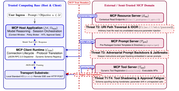
Fig. 3. Architectural decomposition, trust boundaries, and protocol threat vectors in Model Context Protocol (MCP) deployments. Solid blue containers enclose the Trusted Computing Base (Host application and Client runtime); dashed purple containers denote standalone, semi-trusted MCP servers exposing Resources, Prompts, and Tools across the perimeter. Red dashed annotations and boxes isolate primary exploit classes: (T1) tool schema poisoning and tool shadowing during dynamic registration ( tools/list ), (T2) resource URI path traversal and IDOR ( file:///etc/passwd ), (T3) adversarial template injection and sleeper jailbreaks via server-supplied prompts, and (T4) host-level approval fatigue leading to uninspected parameter execution during tool invocation ( tools/call ).
