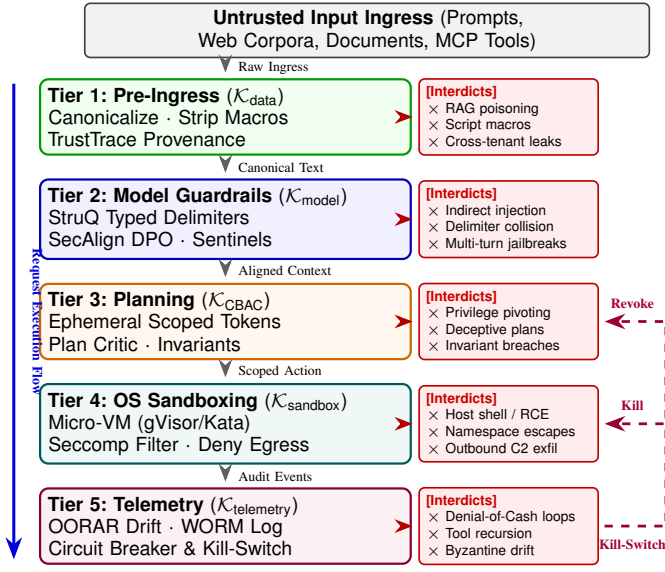
Fig. 5. Multi-Layered Defense-in-Depth framework for Agentic AI across five operational tiers. Distinct container colors identify defense zones ( K_{data} through K_{telemetry} ); red pill badges denote specific threat vectors intercepted at each security boundary; central solid arrows trace downward request traversal from raw ingress to execution; dashed purple loops depict the out-of-band telemetry feedback bus triggering dynamic capability token revocation and sandbox termination upon anomaly detection. By establishing decoupled, defense-in-depth enforcement across all five tiers, the architecture prevents single-point compromise from escalating to systemic control.
