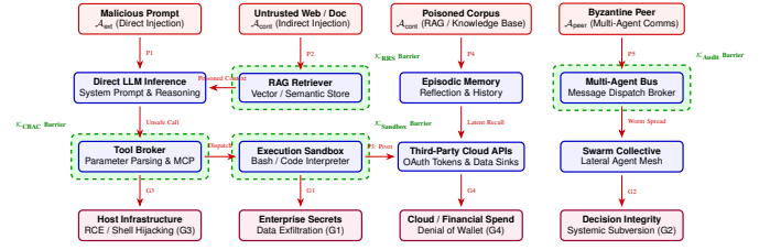
Fig. 2. Causal Threat Graph modeling end-to-end exploit propagation across canonical paths P1, P2, P3, P4, and P5 toward high-value target assets G1–G4. Red boxes denote adversary footholds; blue containers represent internal reasoning and execution substrates; purple boxes represent impact assets. Solid red arrows depict exploit vectors; green dashed contours designate defense interdiction cut barriers positioned on the background layer to sever the kill chain prior to environmental impact.
