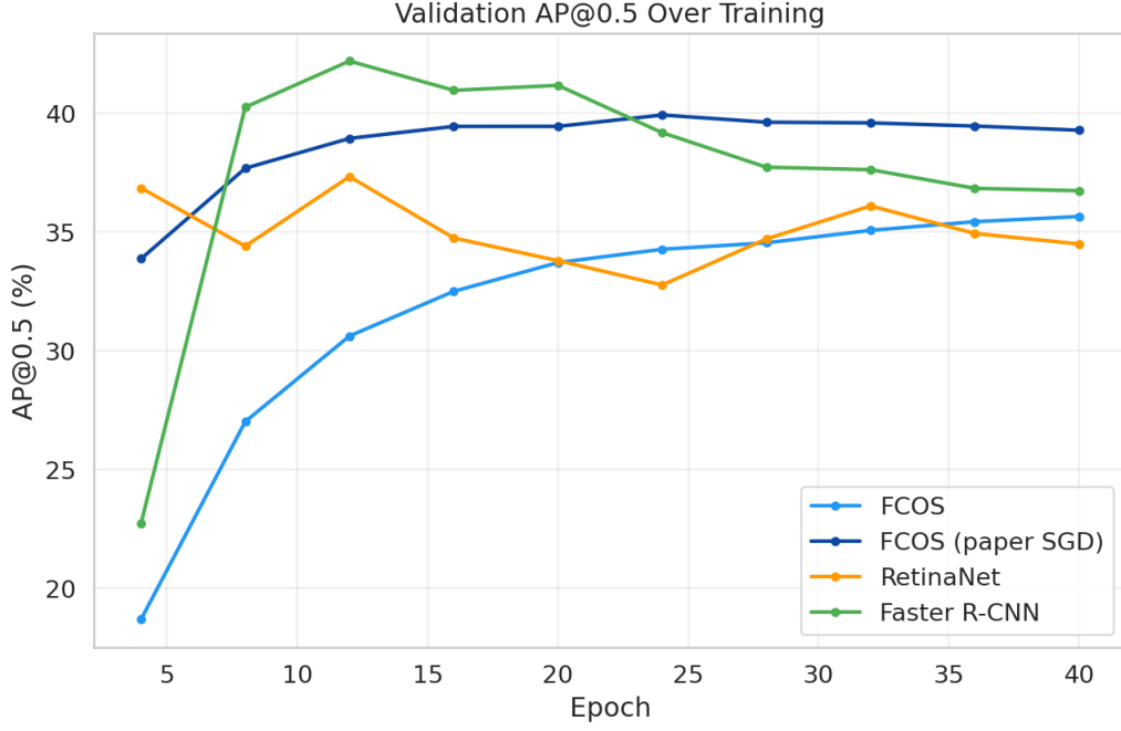
Figure 2: Validation AP@0.5 over training, computed without TTA/Soft-NMS (the headline Table ?? adds those at evaluation time). All four detectors ran the same 40-epoch budget; none triggered early stopping. The peak EMA checkpoint of each detector is the one used at evaluation: epoch 40 for FCOS-Adam, 24 for FCOS paper-SGD, 12 for both RetinaNet and Faster R-CNN.
