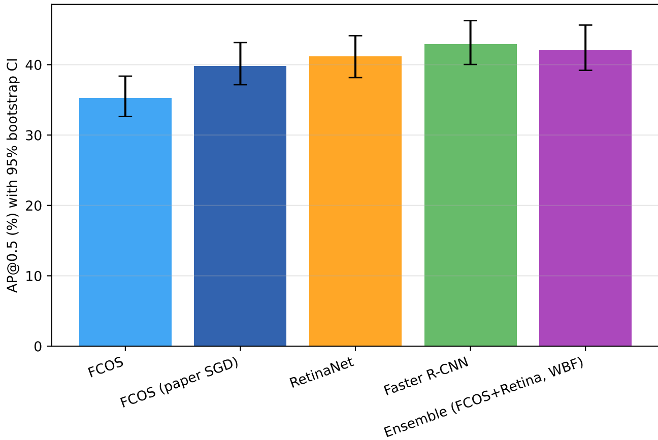
Detection AP@0.5 with patient-level bootstrap CIs (n=500)
