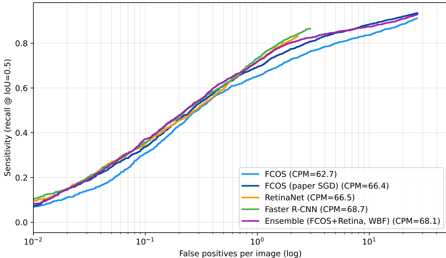
FROC curves on RSNA validation
