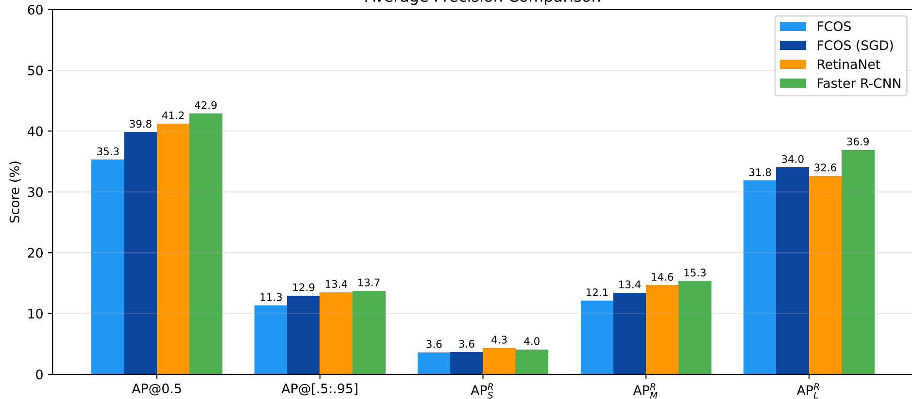
Average Precision Comparison
