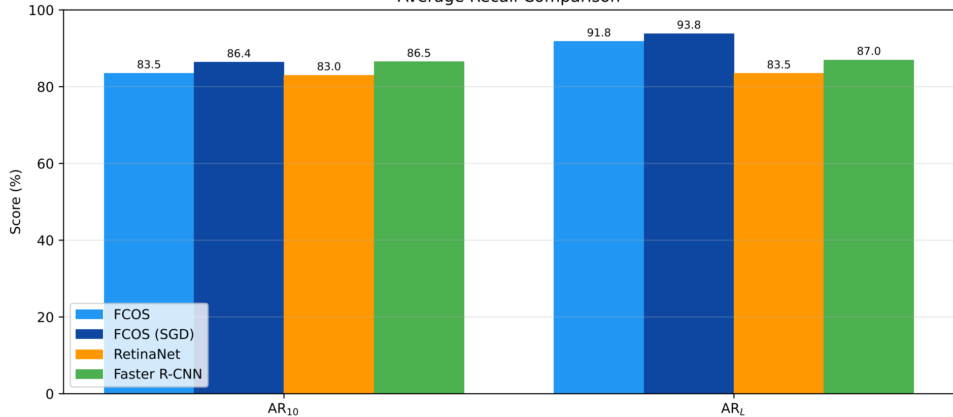
Average Recall Comparison
