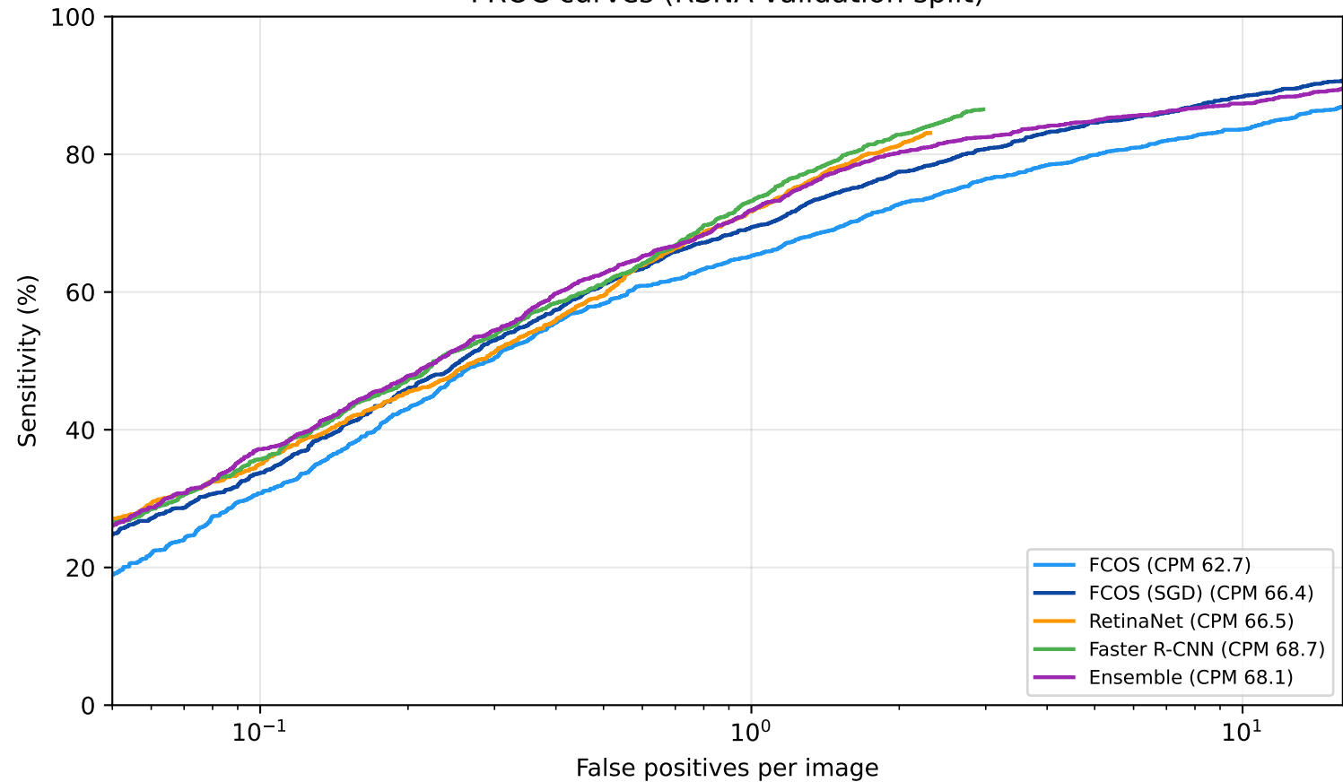
FROC curves (RSNA validation split)
