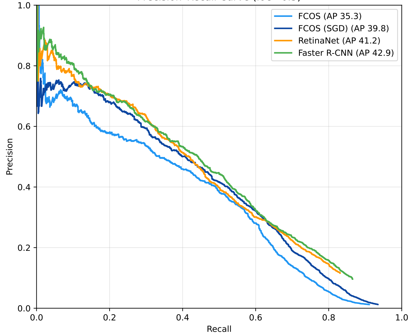
Precision-Recall Curve (IoU=0.5)
