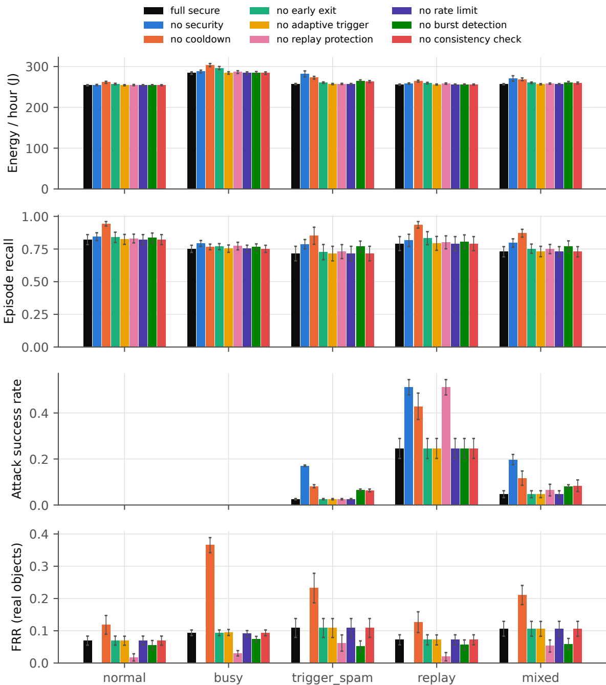
Fig. 12 Ablation: secure system with one component removed (mean, 95% CI)
