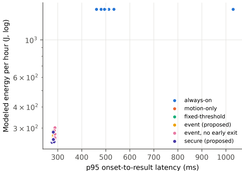
Fig. 8 Energy-latency trade-off (one point per scenario)
