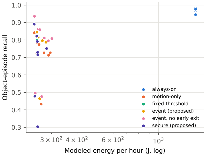
Fig. 9 Detection quality vs modeled energy (one point per scenario)
