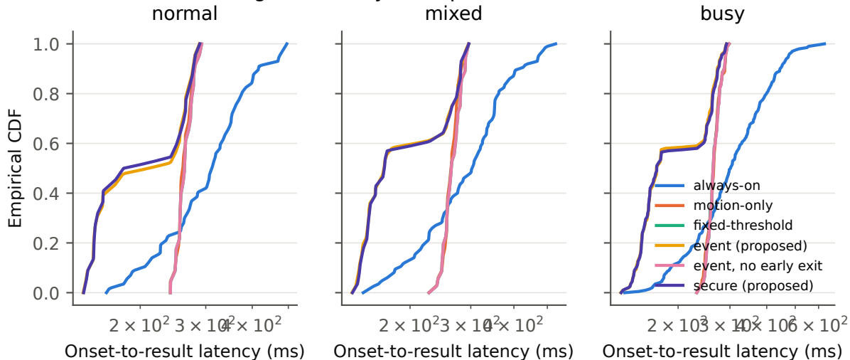
Fig. 3 Latency CDF (pooled over seeds)
