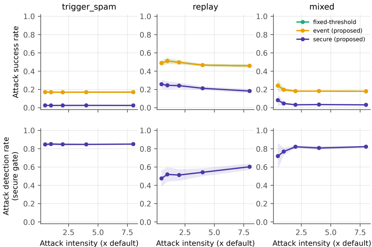
Fig. 7 Security effectiveness vs attack intensity (mean, 95% CI)
