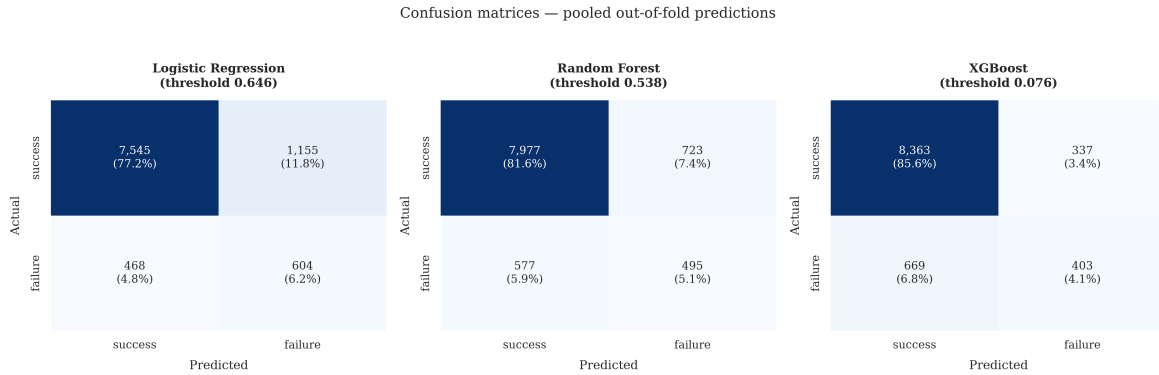
Figure 7.3: Confusion matrices for the three classifiers, computed on pooled out-of-fold predictions and thresholded at each model's mean validation-selected threshold. The operating trade-off is visible directly in the off-diagonal counts: Logistic Regression recovers 604 of the 1,072 failures at the cost of 1,155 false alarms, whereas XGBoost recovers 403 at the cost of 337.
