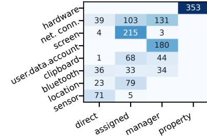
(a) Category x detector
