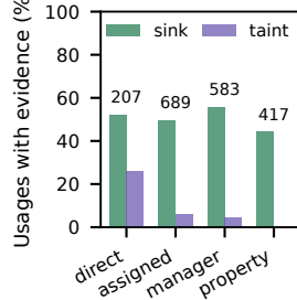
(c) Detector evidence
