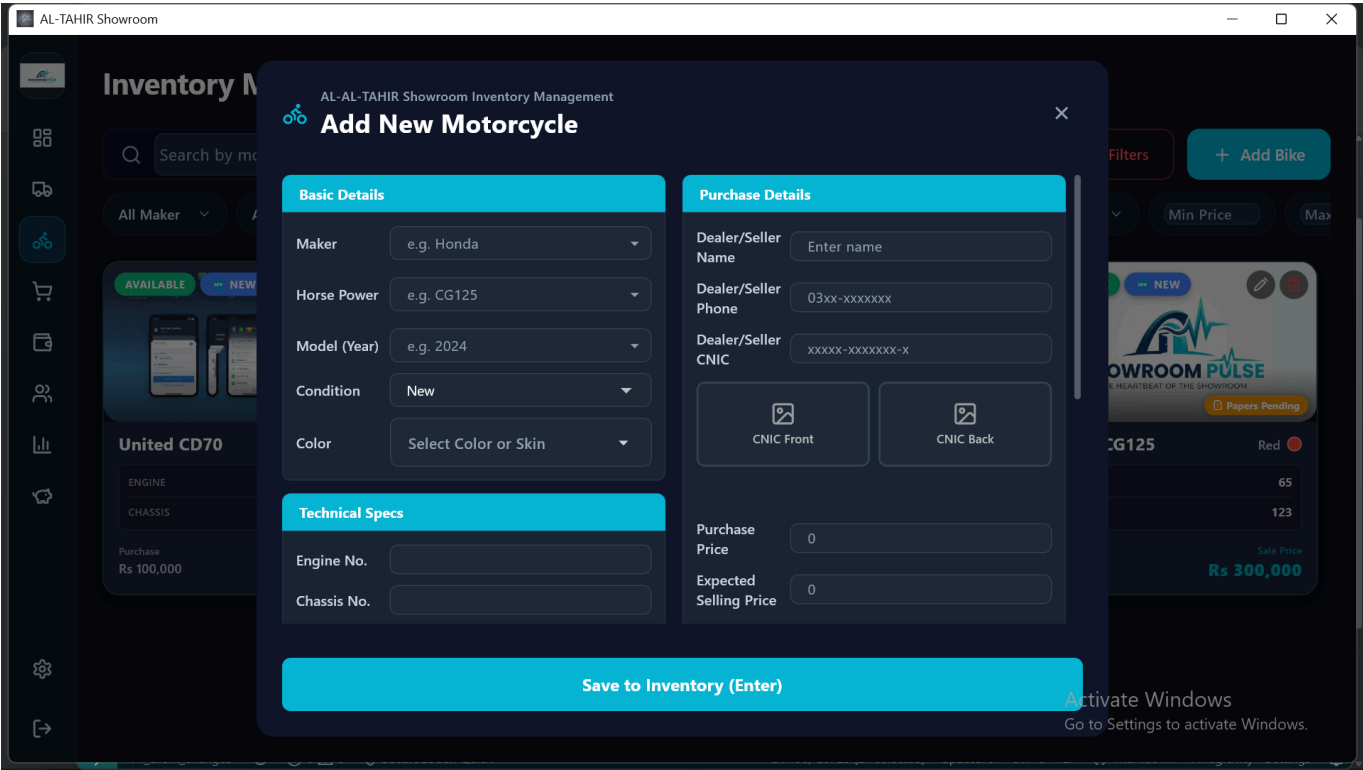
Caption: Comprehensive asset tracking with detailed specifications, pricing configurations, and image handling.
