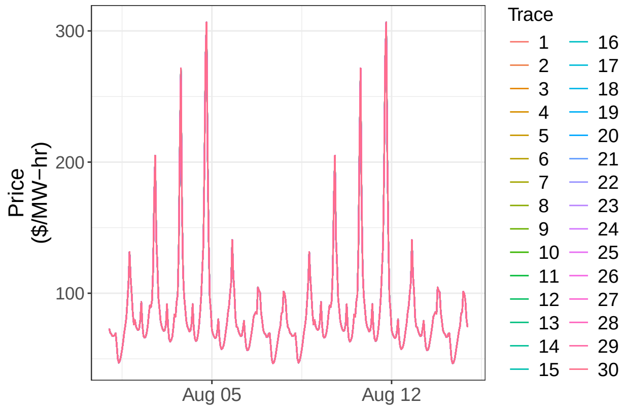
Figure 4. Time series of prices for all traces for the first two weeks of August 2024.
