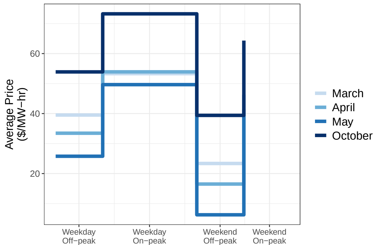
Figure 13 - Average On-peak and off-peak prices for weekdays and weekends of first week of March, April, May, and October.
