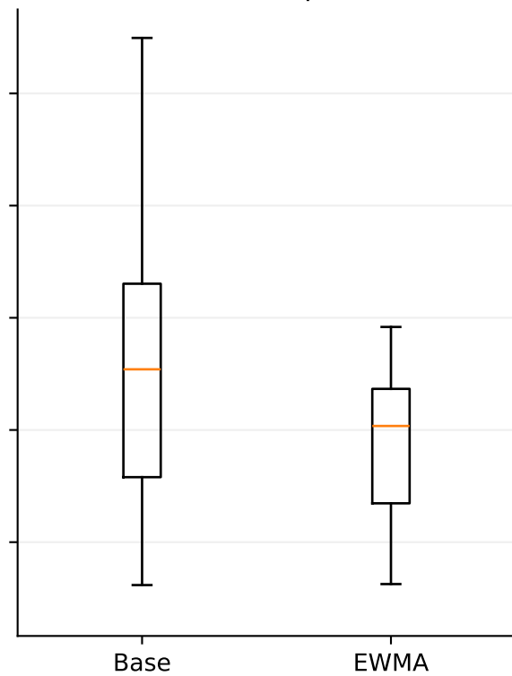
NeuralProphet
