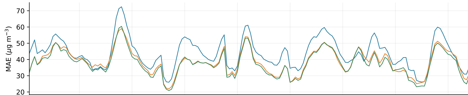
Prophet
