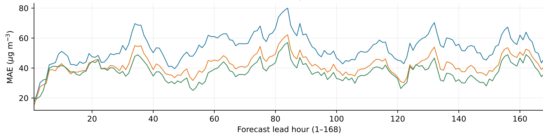
NeuralProphet
