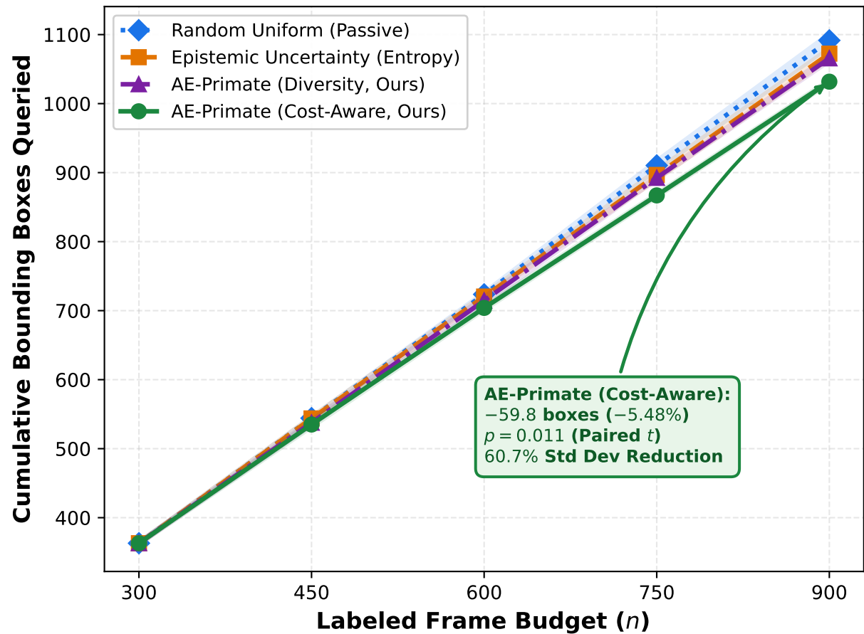
(b) Bounding Box Economy & Variance Suppression
