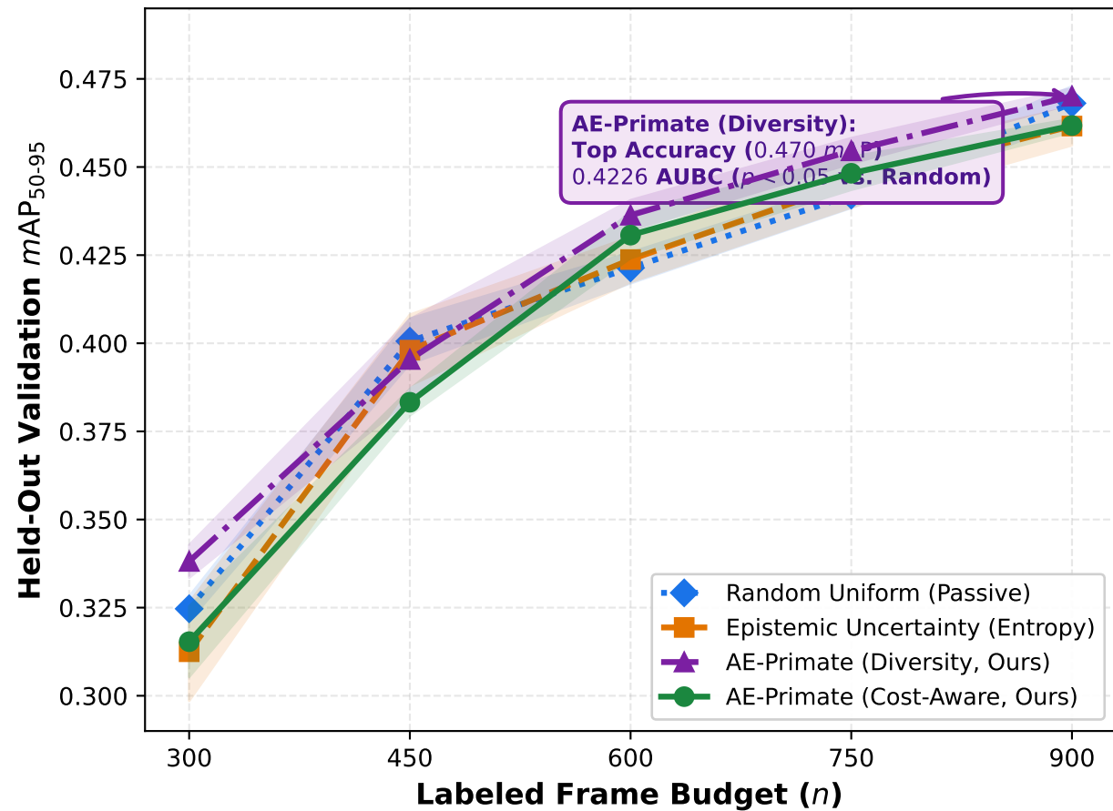
(a) Multi-Cycle Accuracy & OOD Generalization
