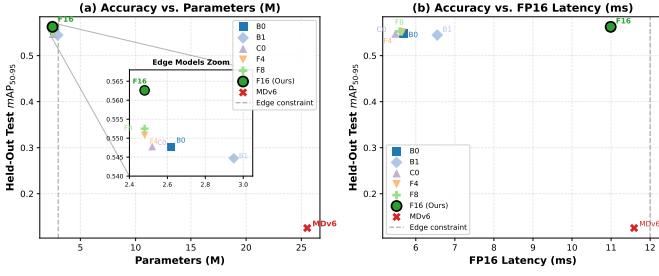
Fig. 1. Accuracy vs. Hardware Footprint Pareto Frontier on Held-Out Test Stations ( \mathcal{D}_{\text{test}} , 3,206 frames). (a) mAP_{50-95} vs. parameter count with embedded edge models inset ([2.40M, 3.05M] \times [0.540, 0.568]) ; (b) mAP_{50-95} vs. FP16 inference latency on NVIDIA A40. Dashed lines mark the edge deployment boundary ( \leq 3.0M parameters, \leq 12.0ms latency).
