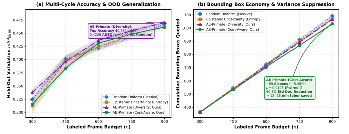
Fig. 2. Multi-Cycle Active Learning Trajectories on Held-Out Validation Stations ( \mathcal{D}_{\text{val}} : 5,560 frames, Mean \pm SEM over N = 5 independent seeds). (a) m\text{AP}_{50-95} vs. labeled frame budget, demonstrating validation accuracy leadership by AE-Primate (Diversity); (b) Cumulative bounding boxes queried vs. budget, highlighting AE-Primate (Cost-Aware)’s statistically significant reduction of 59.8 bounding boxes ( -5.48\% , paired t -test p = 0.0105 ) and 60.3% standard deviation reduction (84.2% variance reduction).
