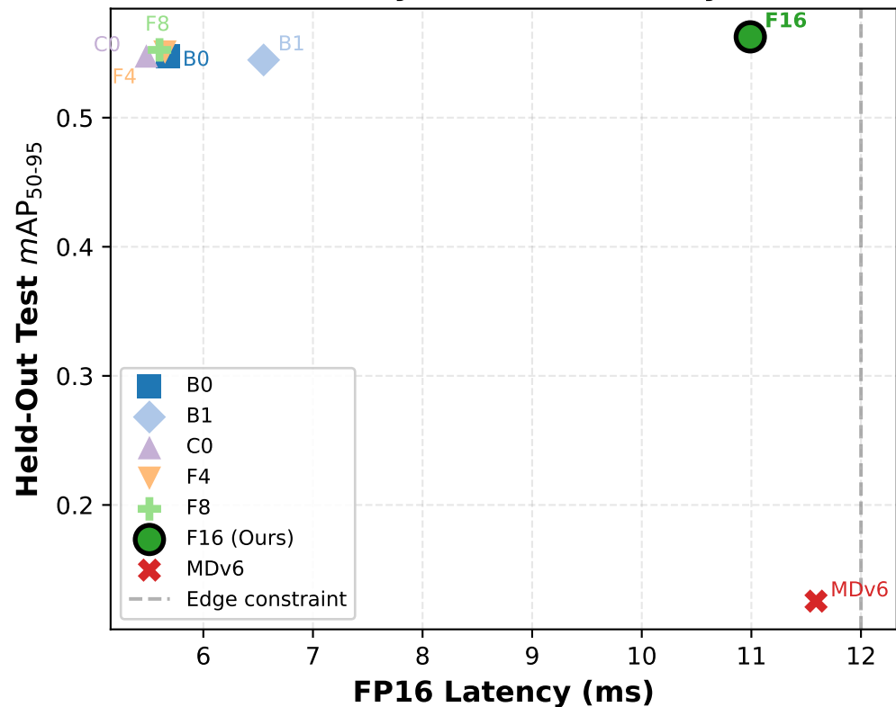
(b) Accuracy vs. FP16 Latency (ms)
