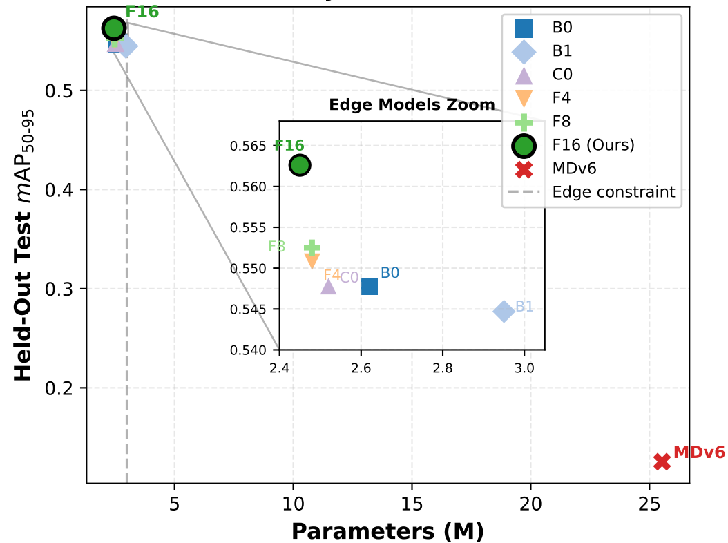
(a) Accuracy vs. Parameters (M)
