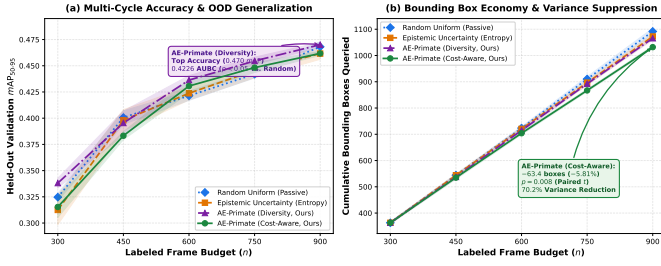
Fig. 2. Multi-Cycle Active Learning Trajectories on Held-Out Validation Stations ( \mathcal{D}_{\text{val}} , 5,560 frames, Mean \pm SEM over N = 5 independent seeds). (a) mAP_{50-95} vs. labeled frame budget, demonstrating accuracy leadership by AE-Primate (Diversity); (b) Cumulative bounding boxes queried vs. budget, highlighting AE-Primate (Cost-Aware)’s statistically significant reduction of 63.4 bounding boxes ( -5.81\% , paired t -test p = 0.008 ) and 70.2% variance reduction.
