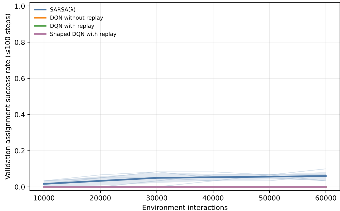
Figure 1. Learning curves (3-checkpoint centered moving average)
