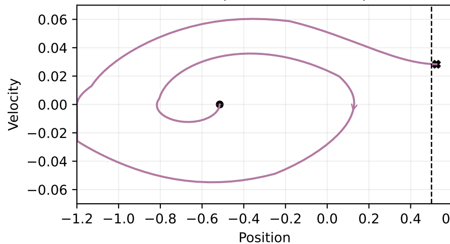
Shaped replay DQN (completion) seed 0, episode 1, 169 steps
