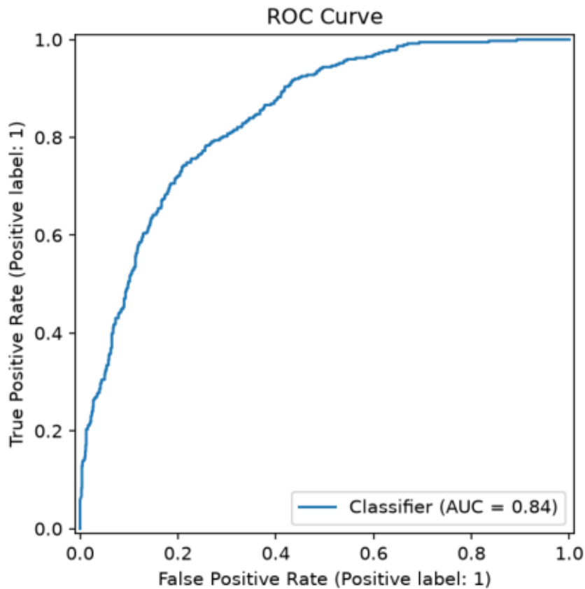
Roc Curve
