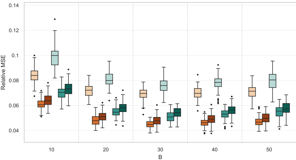
(c) Forecast | Linear
