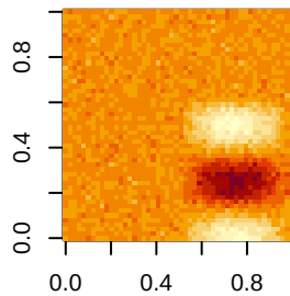
Noisy image
