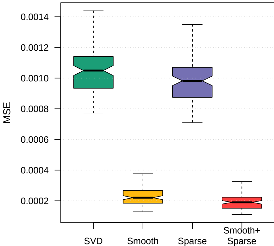
Distribution of MSE by Method
