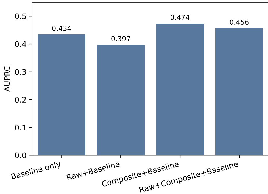
Ablation (Full=7 raw dims): AUPRC
