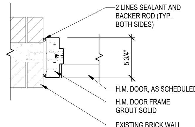
6 DOOR JAMB - HM DOOR @ BRICK A-602 SCALE: 1 1/2" = 1'-0"
