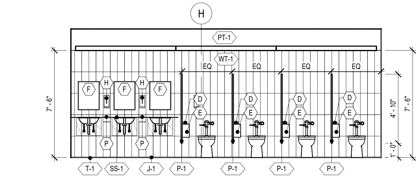
6 A-112 WOMENS RESTROOM SCALE: 1/4" = 1'-0"
