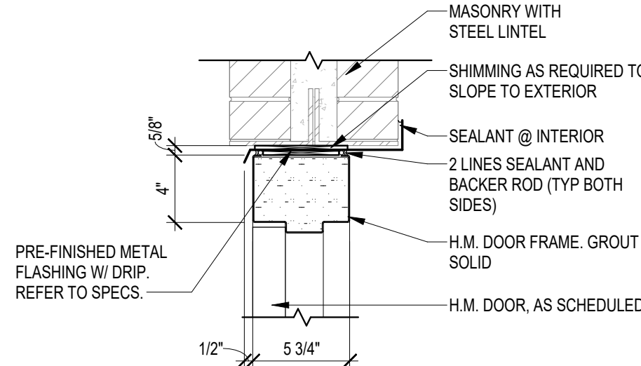
3 DOOR HEAD - HM DOOR @ BRICK A-602 SCALE: 1 1/2" = 1'-0"
