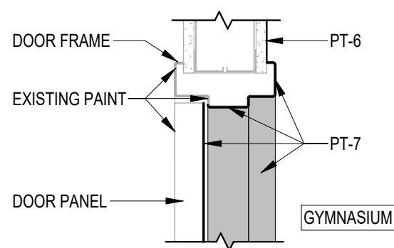
DOOR FRAME PAINT SCALE: 1 1/2" = 1'-0"
