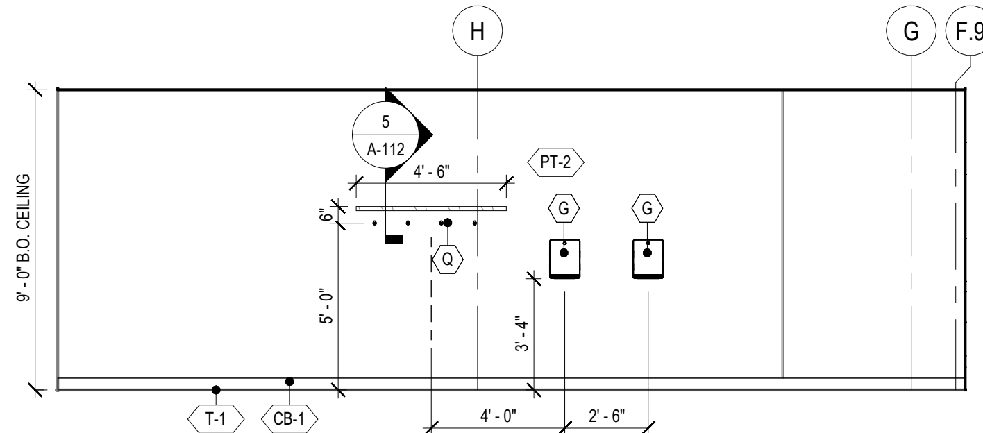
8 A-112 WOMENS RESTROOM SCALE: 1/4" = 1'-0"
