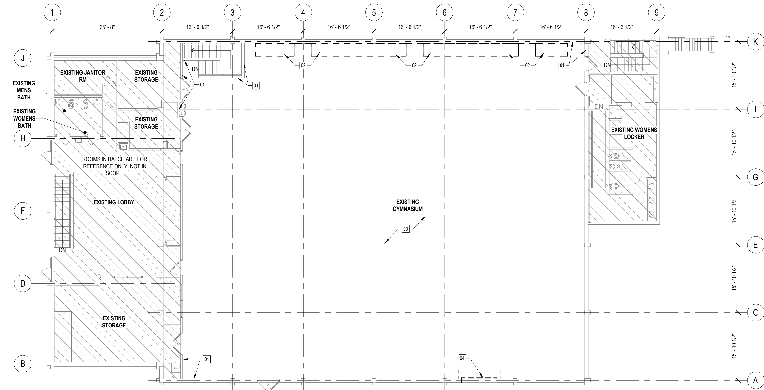
DEMOLITION - GYMNASIUM SCALE: 3/32" = 1'-0" TRUE NORTH BLDG NORTH
