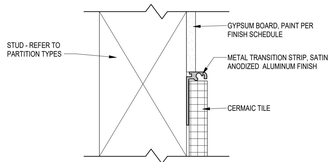
14 A-112 TRANSITION DETAIL - TILE TO GYP. SCALE: 3" = 1'-0"
