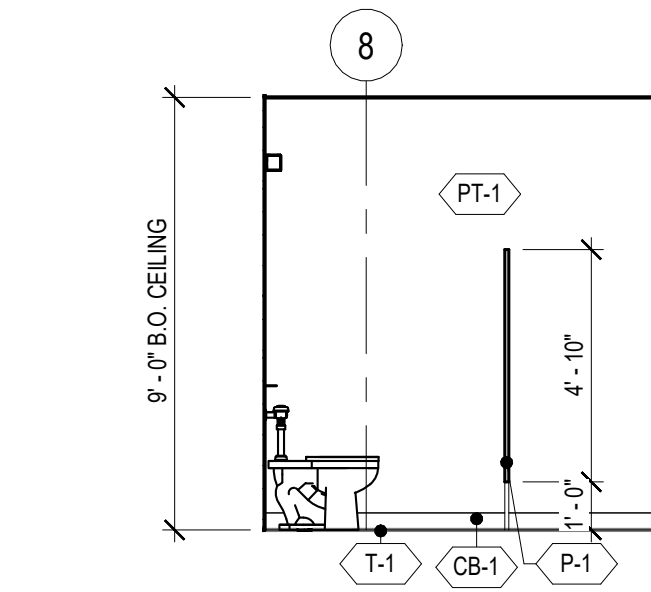
7 A-112 WOMENS RESTROOM SCALE: 1/4" = 1'-0"
