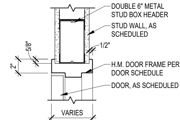
4 DOOR HEAD - HM DOOR @ GWB A-602 SCALE: 1 1/2" = 1'-0"
