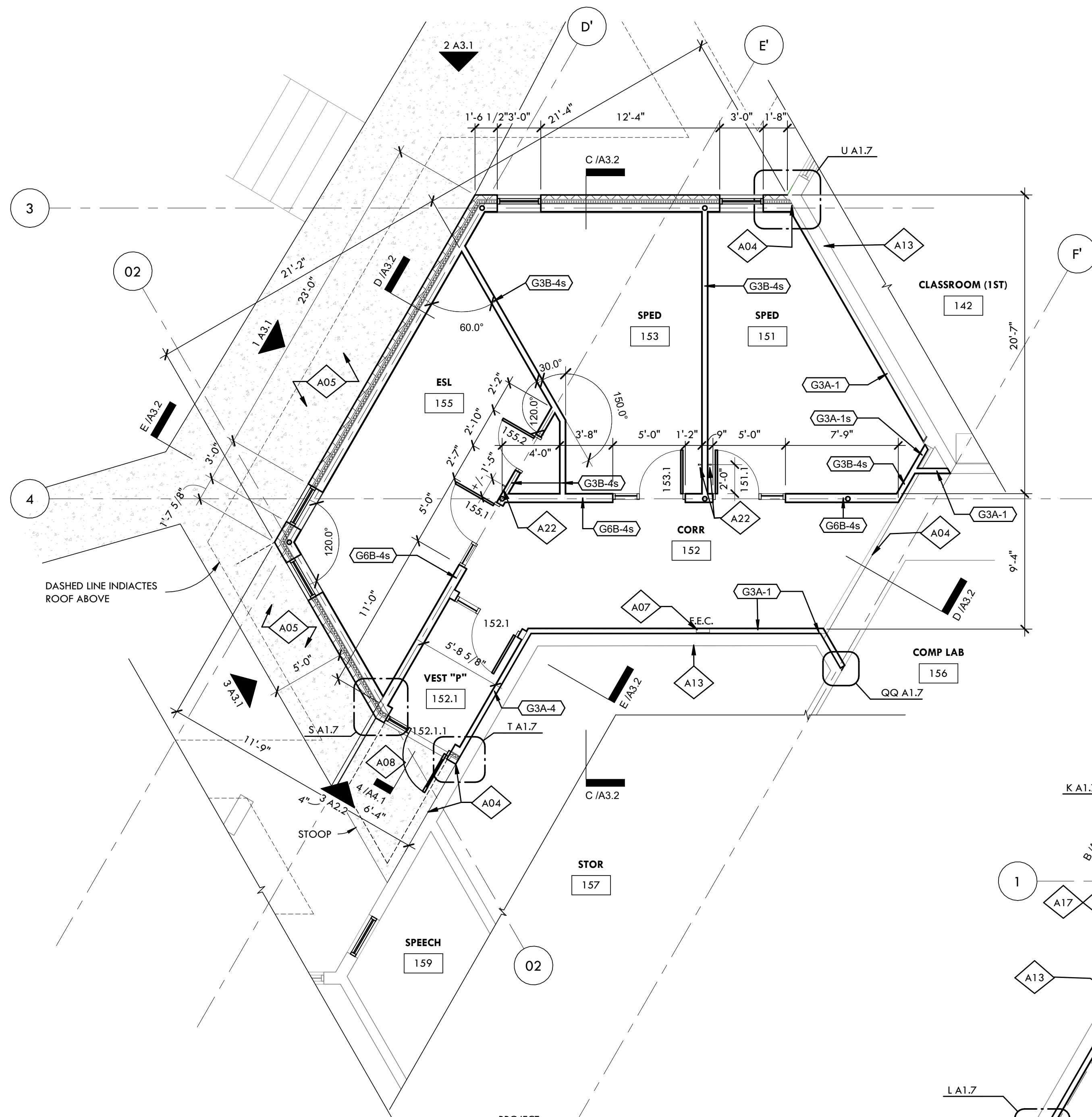
1 ENLARGED PLAN - ADDITION 2 SCALE: 3/16" = 1'-0"
