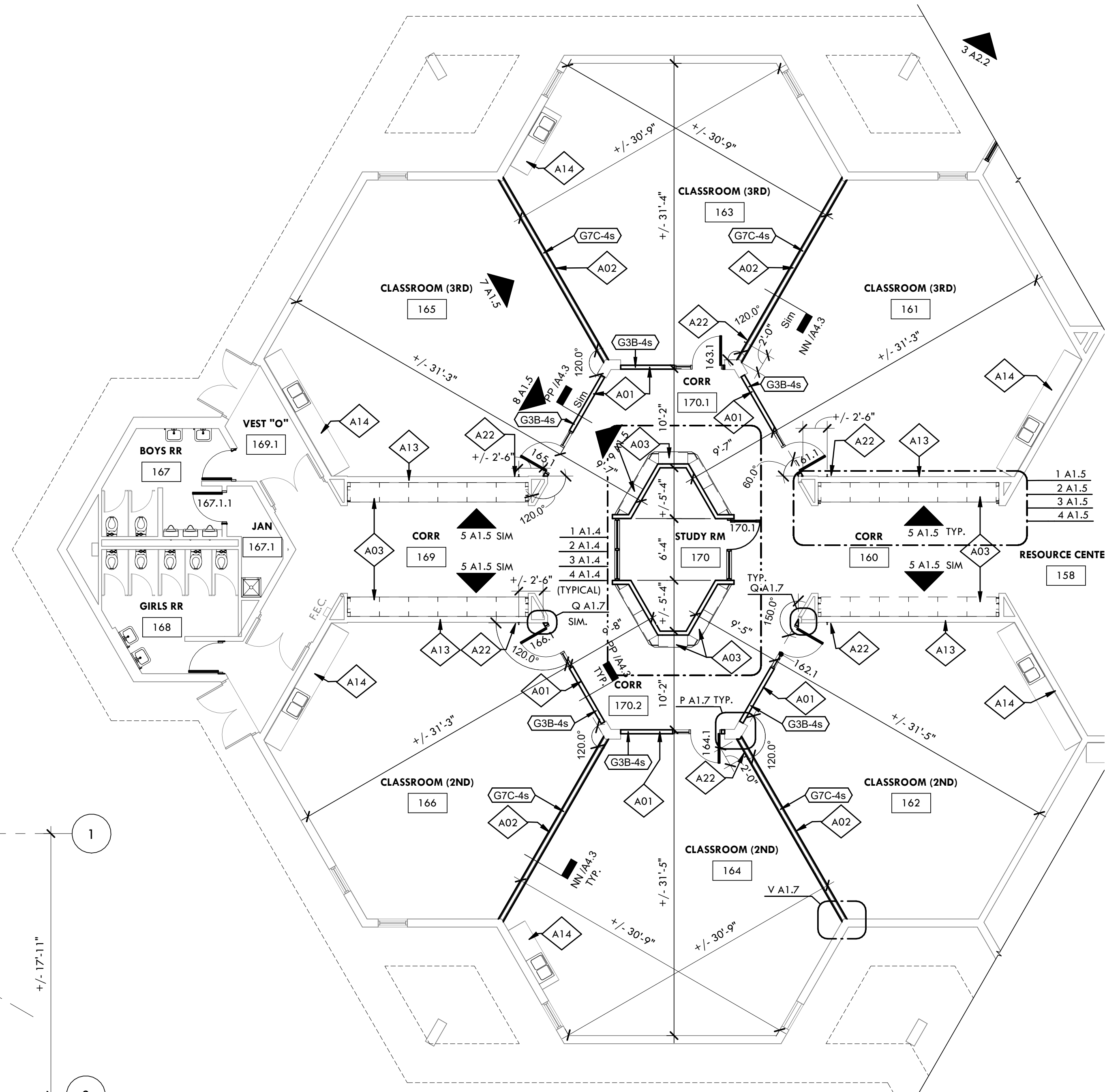
2 ENLARGED PLAN - CLASSROOM CLUSTER (TYPICAL OF 3) SCALE: 1/8" = 1'-0"
