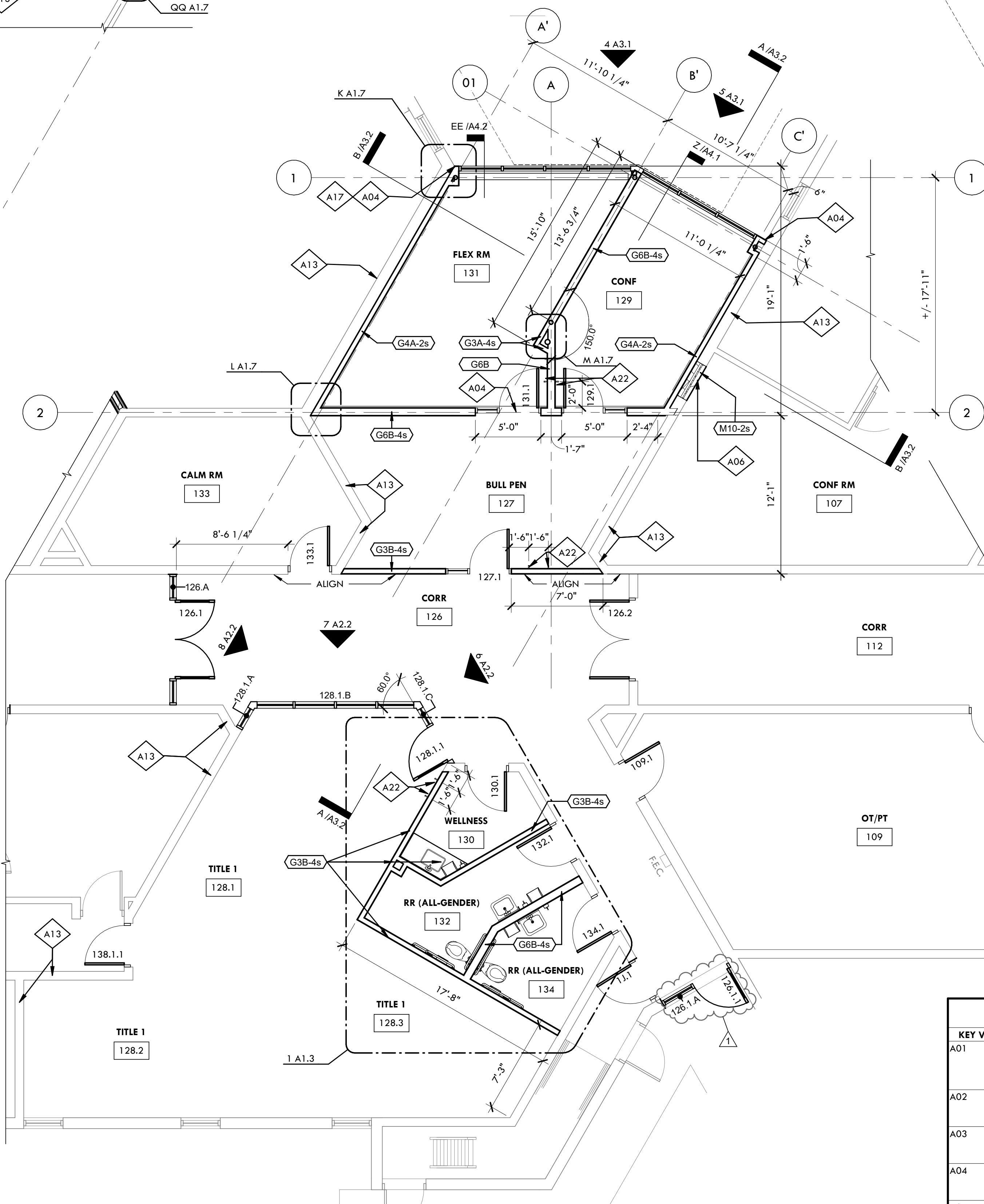
3 ENLARGED PLAN - ADDITION 1 & CORE OFFICES SCALE: 3/16" = 1'-0"
