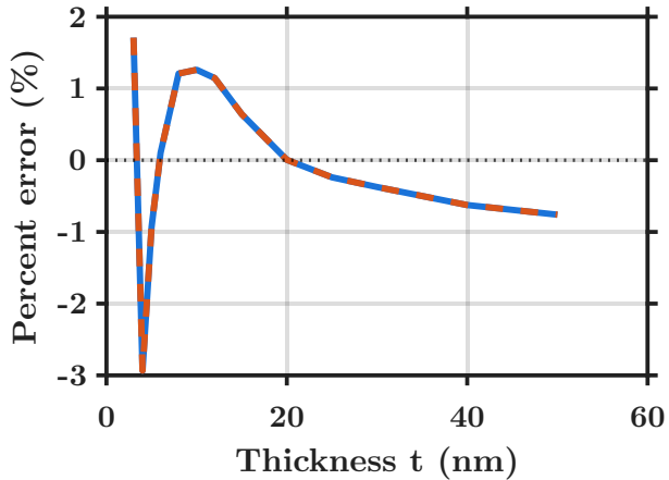
Fit Error vs Thickness
