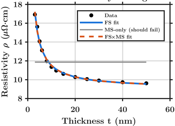
Ru Resistivity Scaling
