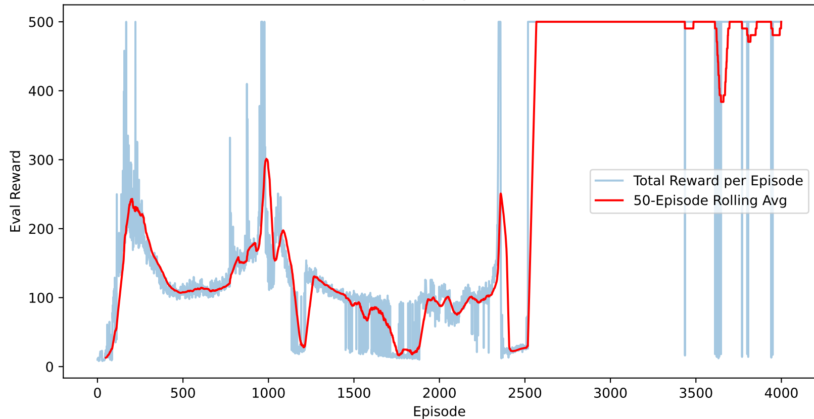
CartPole DQN Training Progress (Eval Rewards)
