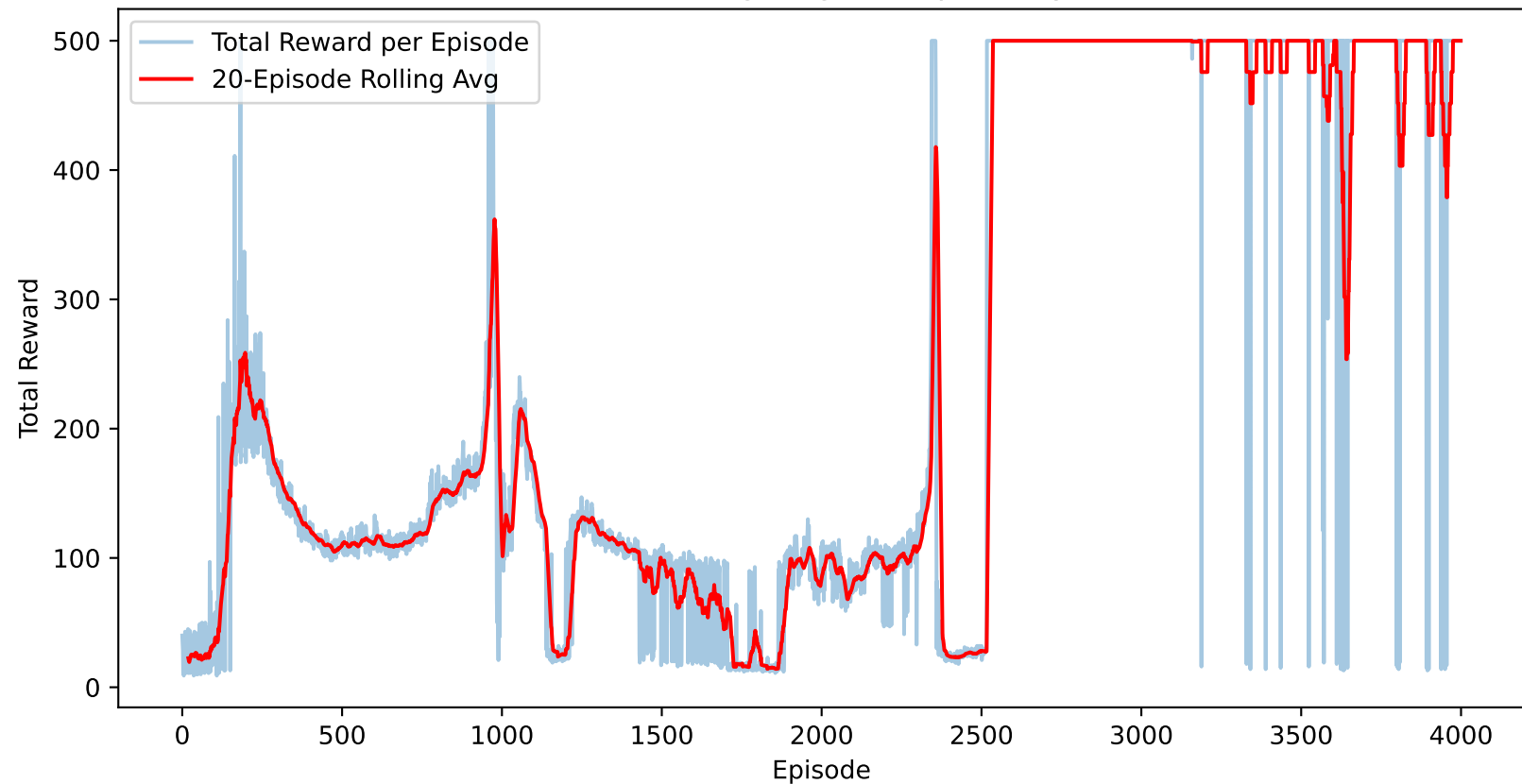
CartPole DQN Training Progress (Eps-Policy Rewards)
