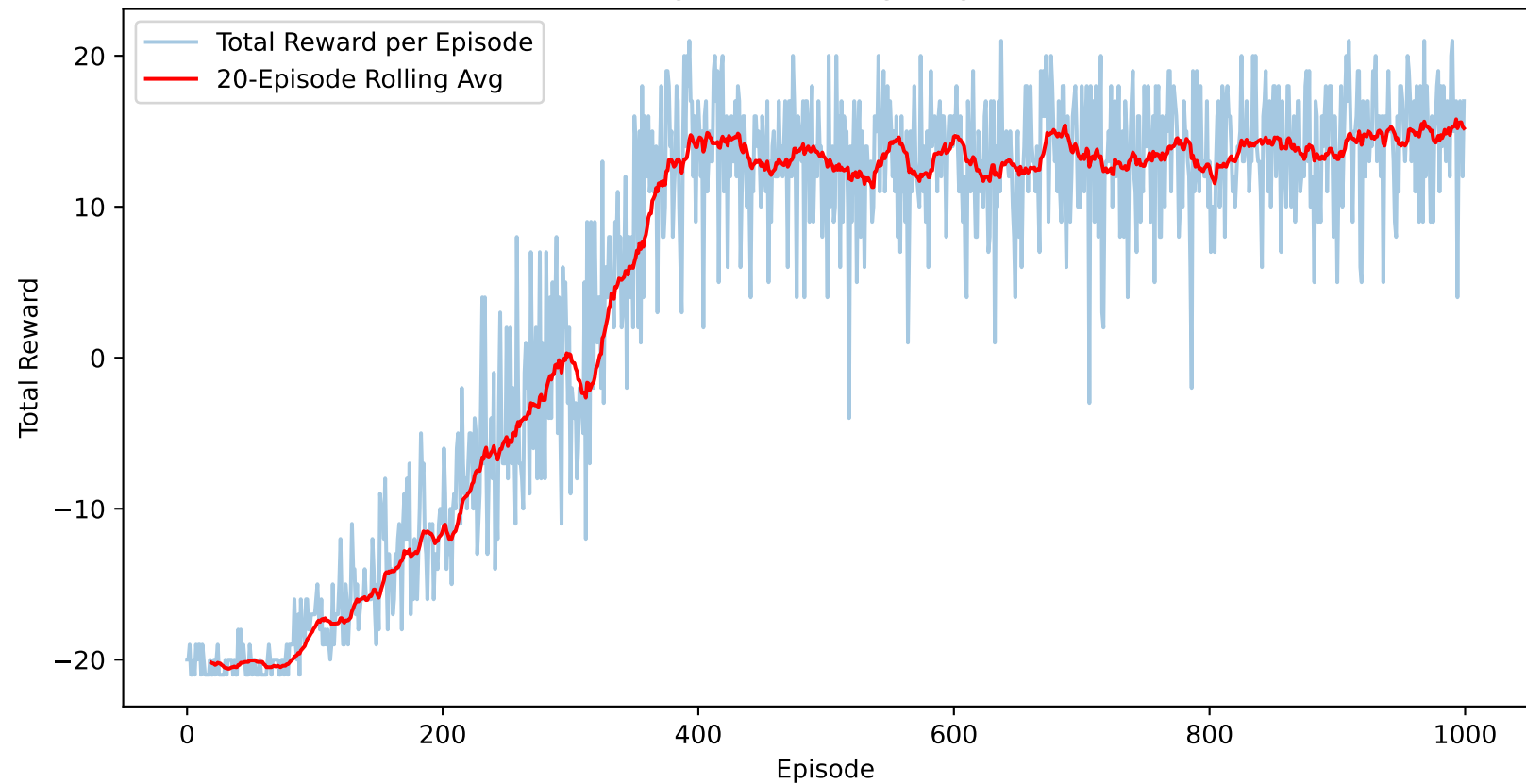
Pong DQN Training Progress
